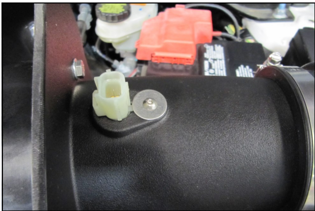
10. Transfer the factory Air Temperature Sensor into the Airaid Intake tube and align the sensor tab with the Groove in the tube. Secure the sensor to the tube using the 8-32 Button Head Bolt and the 3/4" washer.
