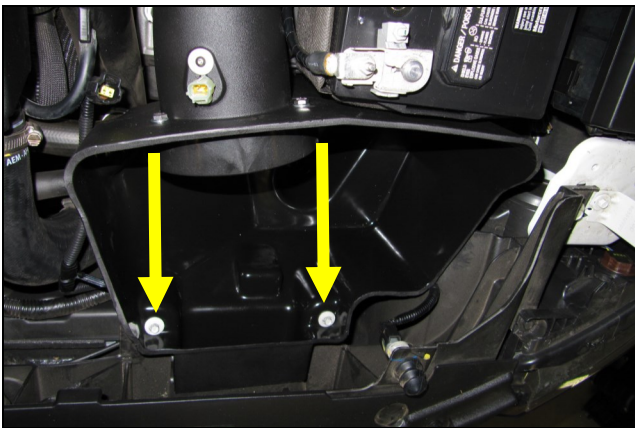
11. Place the Airaid Intake assembly in the original location of the Factory Air box and secure using the factory hardware from step 4. Slide the coupler and clamps onto 90 deg. Elbow pipe and tighten the clamps.
