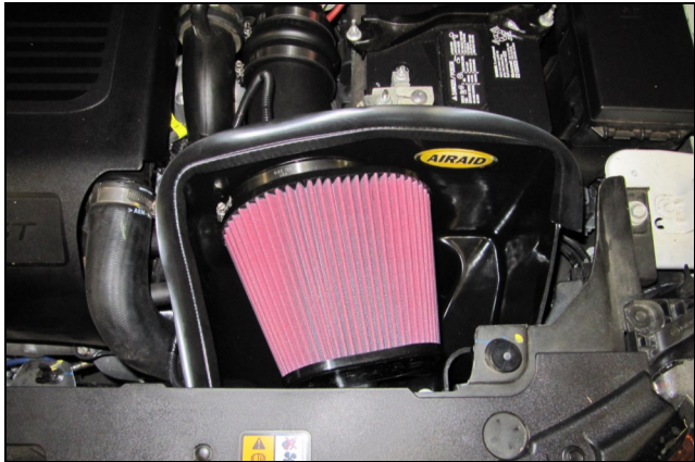
15. Install the Airaid Premium filter onto the Filter Adapter and tighten the clamp. Install the weather strip onto the top of the Air box as shown, with the contour rolling away from the filter.
