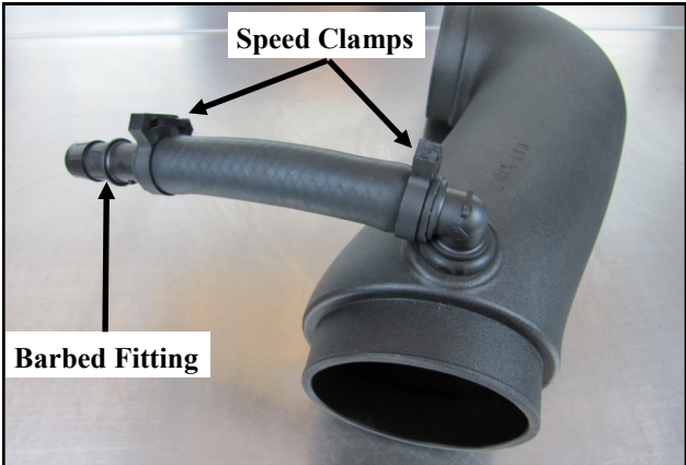
10. Insert the Barbed Fitting into the supplied PCV Hose and connect it to the Elbow in the Intake Tube. Use the Speed Clamps to secure the Hose onto the Fittings.
